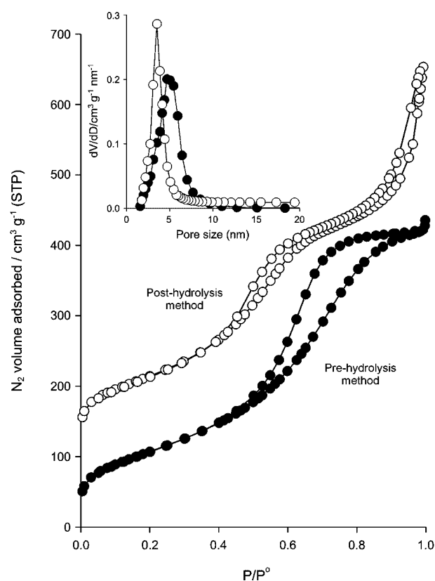
Fig. 1. N 2 adsorption-desorption isotherms of mesoporous aluminas, AlS-1 and AlS-5, prepared by pre-(◆) and post-(○) hydrolysis method. BJH pore sizes obtained from the desorption isotherms are included for comparison (insert figure).
